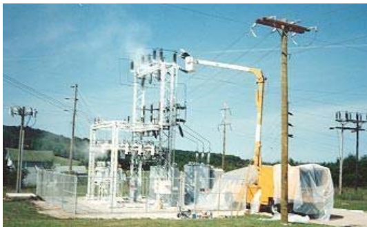
Painting Substation
